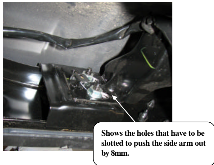
FIG 3: Driver side arm of bumper step shown
